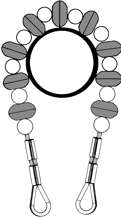
BASKET ANCHOR
